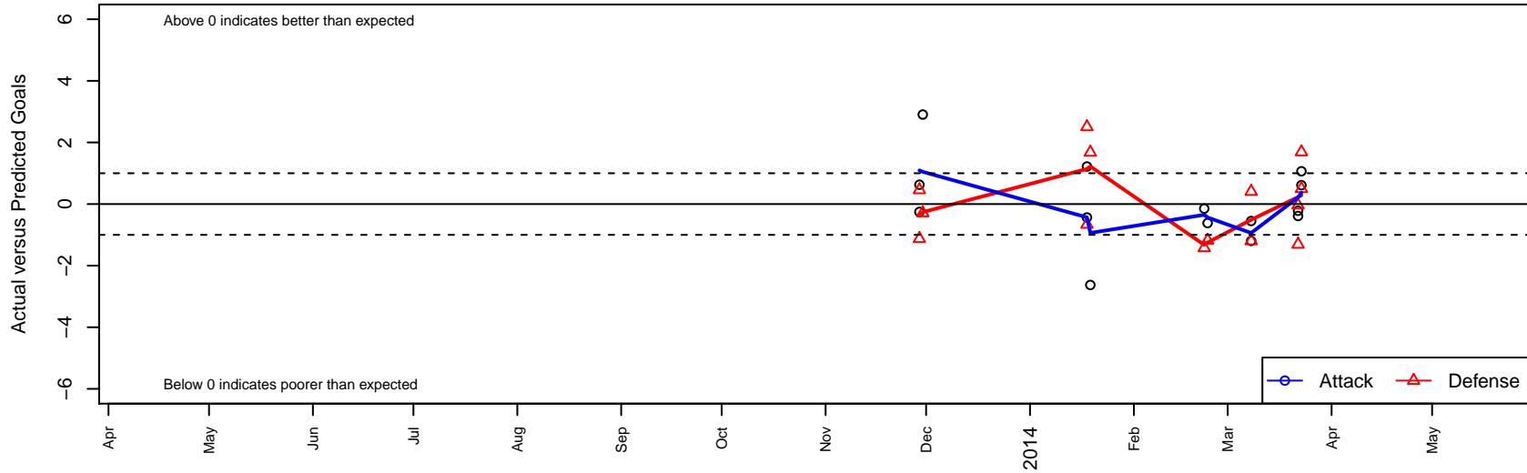
Nomads SC B00 Dots are actual minus expected GF (blue circles) and GA (red triangles). Blue line is smoothed change in attack strength. Red is smoothed change in defense strength.
